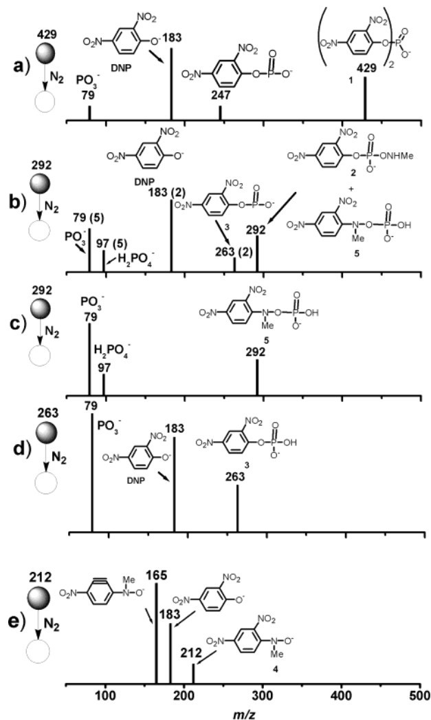
FIGURE 7. ESI-MS/MS spectra after CID of anionic intermediates observed in the reaction of 0.01 M BDNPP with 0.1 M MeNH 2 OH in aqueous methanol (50% v/v) at pH 10 for ions of m/z 429, 292, 263, and 212.
