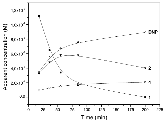
FIGURE 5. Apparent concentrations of main products of the reactions of 0.01 M BDNPP with 0.1 M NHMeOH, in D 2 O, pH 9, and 25 °C: (■) 1 , (Δ) DNP, (▼) 2 , and (○) 4 .
