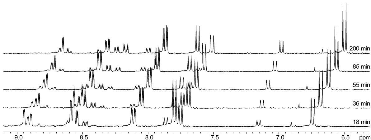
FIGURE 3. ^1\text{H} NMR spectra of the reaction mixture of 0.01 M BDNPP with 0.1 M NHMeOH, in \text{D}_2\text{O} , pD 9, and 25 °C. See Table 2 for identification of signals.
