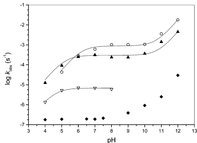
FIGURE 1. Plots of \log k_{\text{obs}} versus pH for nucleophilic attack on BDNPP by MeNHOH (O), (\text{Me})_2\text{NOH} (▲), \text{NH}_2\text{OMe} (▽), and \text{H}_2\text{O} (◆), at 25 °C.
