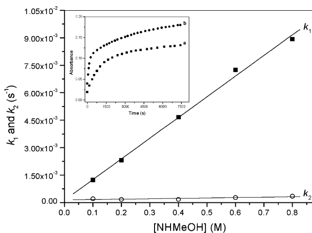
FIGURE 2. Plots of k_1 (■) and k_2 (○) as a function of [\text{NHMeOH}] for nucleophilic attack on BDNPP, at pH 9 and 25 °C. Inset: kinetic plots for [\text{NHMeOH}] = (a) 0.1 and (b) 0.6 M.
